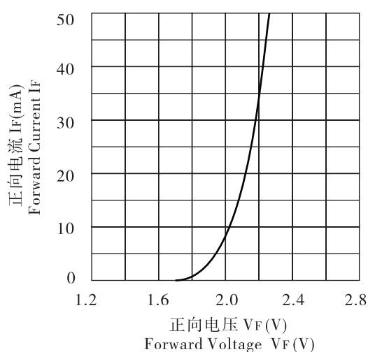
Typical Electro-Optical Characteristic Curves ( Ta=25℃ ) (Red)
