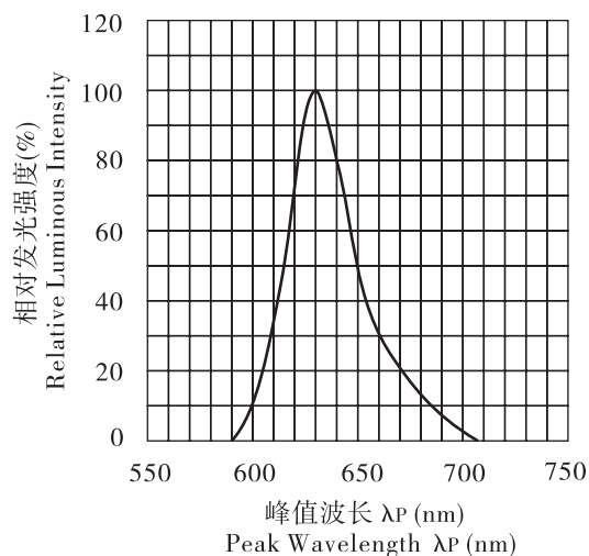
Typical Electro-Optical Characteristic Curves ( Ta=25℃ ) (Red)
