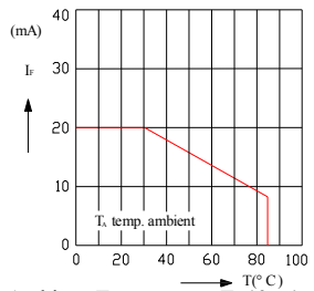
FIG.4 FORWARD CURRENT VS. AMBIENT TEMPERATURE
