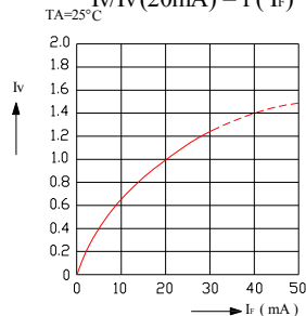
FIG.3 RELATIVE LUMINOUS INTENSITY VS. FORWARD CURRENT
