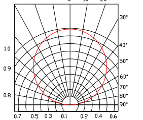
FIG.5 RADIATION DIAGRAM
