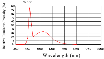
FIG.1 RELATIVE LUMINOUS INTENSITY
