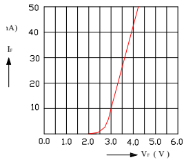
FIG.2 FORWARD CURRENT VS. FORWARD VOLTAGE
