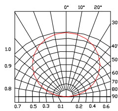
FIG.5 RADIATION DIAGRAM
