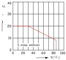
FIG.4 FORWARD CURRENT VS. AMBIENT TEMPERATURE
