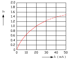
FIG.3 RELATIVE LUMINOUS INTENSITY VS. FORWARD CURRENT
